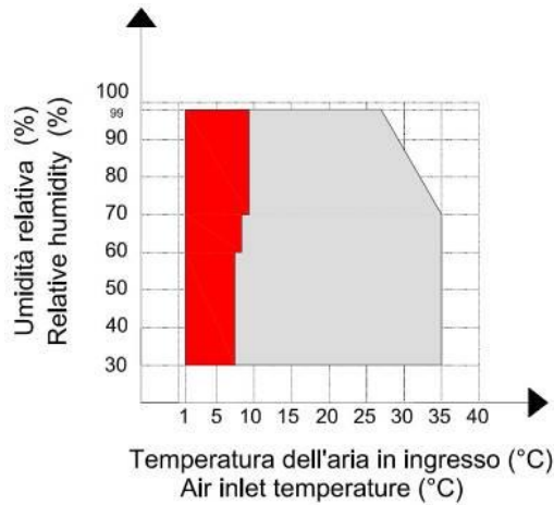
Fig. 2 - Operation table
